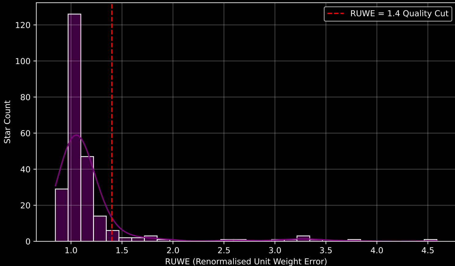
GALAH DR4 Field [9027] RUWE Distribution (n= 240)
