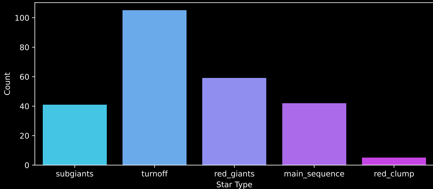
GALAH DR4 Field: [9027] Count plot of Star Type
